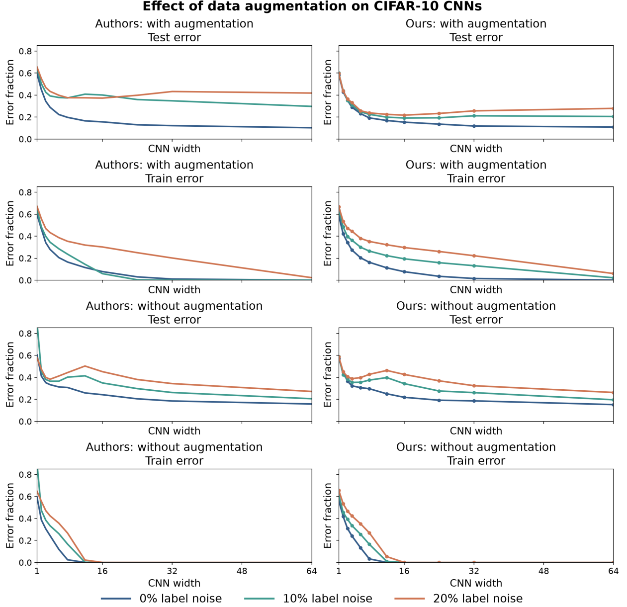
Fig. 5. Effect of data augmentation on CIFAR-10 CNN error, reproducing paper Figure 5. Both sources use the same eleven widths and label-noise rates of 0, 10, and 20%. The left column shows the authors at measurement index 194; the right column shows ours after 50,000 SGD updates. The author point corresponds to approximately 49,920 updates only under the unverified assumption of 256 updates per measurement, so training duration is not confirmed to match.
