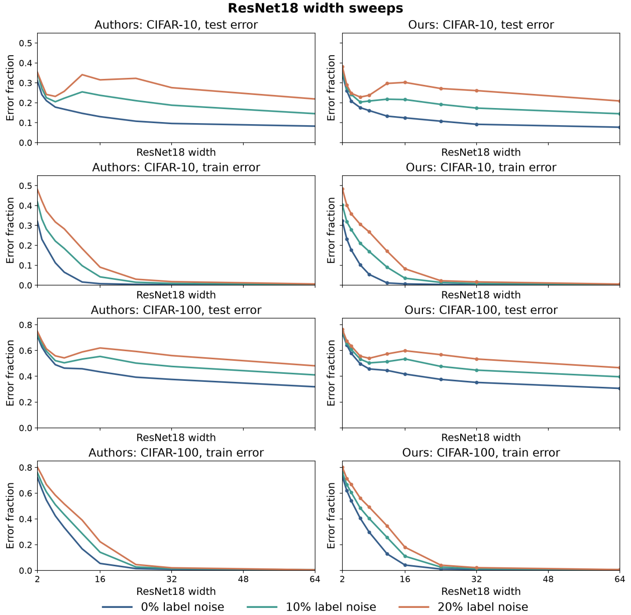
Fig. 4. ResNet18 error versus width on CIFAR-10 and CIFAR-100, reproducing paper Figure 4. Both sources use the same ten widths and label-noise rates of 0, 10, and 20%. The left column shows the authors at displayed epoch 400 (measurement index 399); the right column shows ours at recorded epoch 400.
